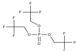
Tris(2,2,2-trifluoroethyl)phosphate
