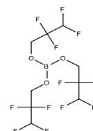
Tris(2,2,3,3-tetrafluoropropyl)borate
