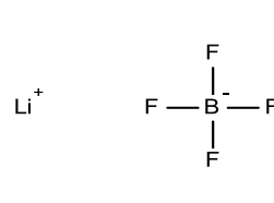
Lithium tetrafluoroborate
