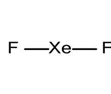
Xenon difluoride, electronic grade
