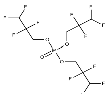
Tris(2,2,3,3-tetrafluoropropyl)phosphate
