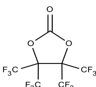
Tetrakis(trifluoromethyl)ethylene carbonate
