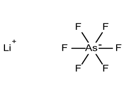
Lithium hexafluoroarsenate
