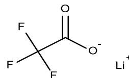
Lithium trifluoroacetate
