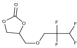
3-(2,2,3,3-Tetrafluoropropoxy)propyl-1-ene carbonate
