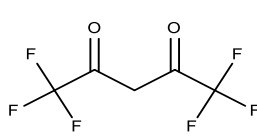
Hexafluoroacetylacetone, electronic grade
