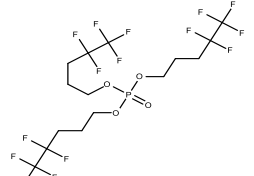
Tris(4,4,5,5,5-pentafluoropentyl)phosphate
