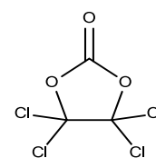
Tetrachloroethylene carbonate
