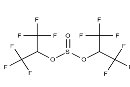
Bis(hexafluoroisopropyl) sulfite
