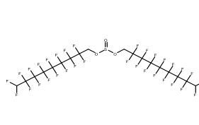
Bis(1H,1H,9H-perfluorononyl) sulfite
