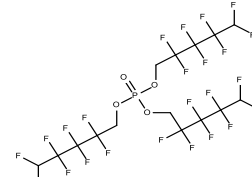
Tris(1H,1H,5H-octafluoropentyl)phosphate
