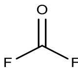
Carbonyl fluoride
