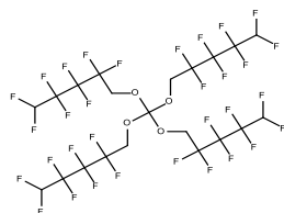
Tetrakis(2,2,3,3,4,4,5,5-octafluoropentyl)orthocarbonate
