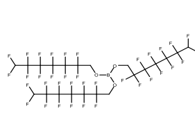
Tris(1H,1H,7H-perfluoroheptyl)borate
