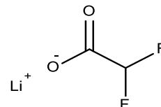
Lithium difluoroacetate
