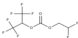
2,2-Difluoroethyl hexafluoro isopropyl carbonate
