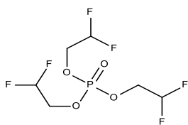
Tris(2,2-difluoroethyl)phosphate
