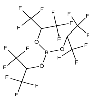
Tris(1,1,1,3,3,3-hexafluoroisopropyl)borate
