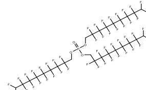
Tris(1H,1H,9H-perfluorononyl)phosphate
