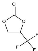
3,3,3-Trifluoropropylene carbonate
