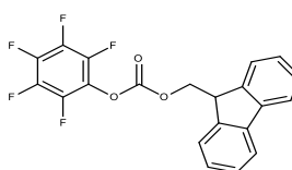
9-Fluorenylmethyl pentafluorophenyl carbonate
