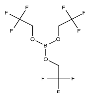
Tris(2,2,2-trifluoroethyl)borate
