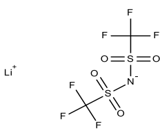
Lithium bis(trifluoromethanesulfonyl)imide
