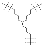
Tris(4,4,5,5,5-pentafluoropentyl)borate
