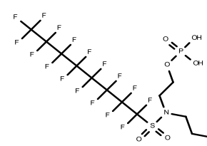
2-[N-Propyl(perfluorooctane sulfonamido)]ethoxyphosphonic acid
