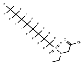
2-N-Ethyl(perfluorooctane sulfonamido)acetic acid
