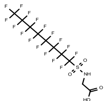
2-(Perfluorooctanesulfonamido) acetic acid
