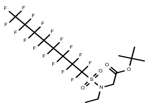
tert-Butyl 2-N-ethyl(perfluorooctane sulfonamido)acetate
