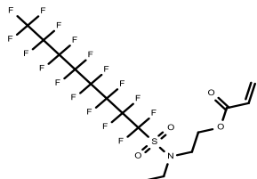
2-(N-Ethylperfluorooctanesulfamido) ethyl acrylate
