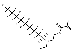
2-(N-Ethylperfluorooctanesulfamido) ethyl methacrylate
