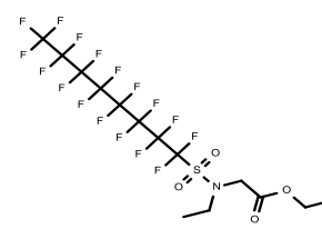
Ethyl 2-[N-ethyl(perfluorooctane sulfonamido)]acetate
