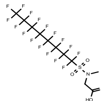
2-N-Methyl(perfluorooctane sulfonamido)acetic acid
