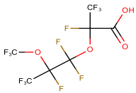
Perfluoro-2,5-dimethyl- 3,6-dioxoheptanoic acid
