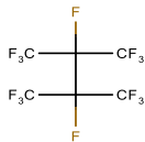
Perfluoro(2,3-dimethylbutane)
