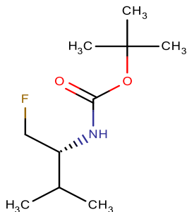
tert-Butyl (R)-(1-fluoro-3- methylbutan-2-yl)carbamate 4156-3-R4 [942275-75-4]
