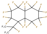
Perfluoro(isopropyl)decalin, mixed isomers
