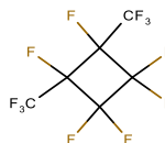
Perfluorodimethylcyclobutane
