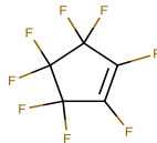
Octafluorocyclopentene
