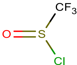
Trifluoromethanesulfinyl chloride 6165-6-00 [20621-29-8]
