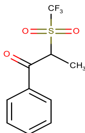
1-Phenyl-2-[(trifluoromethyl) sulfonyl]-1-propanone 6663-3-88 [155201-05-1]
