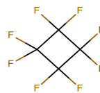
Octafluorocyclobutane
