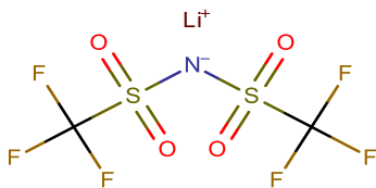
Lithium bis(trifluoromethanesulfonyl)imide 8169-2-01 [90076-65-6]
