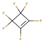
Hexafluorocyclobutene
