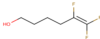
5,6,6-Trifluorohex-5-enol 2301-3-04 [145343-37-9]
