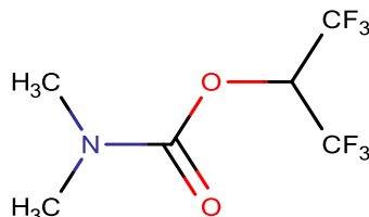
1,1,1,3,3,3-Hexafluoropropan-2-yl N,N-dimethylcarbamate 4148-3-0B [607382-53-6]
