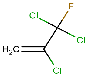
2,3,3-Trichloro-3-fluoro prop-1-ene 1300-7-46 [421-42-1]
