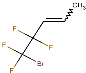
5-Bromo-4,4,5,5-tetrafluoro pent-2-ene 1300-B-0A [22515-91-9]
