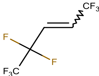
2H,3H-Octafluoro-2-pentene 1300-3-58 [152267-17-9]
