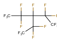
Perfluoro(3-ethylpentane)
