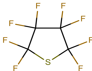
Octafluorotetramethylene sulfide 5H66-2-01 [706-76-3]
